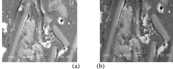
Fig. 4 SEM image of 15% Glass fiber + 5% MoS 2 filled PTFE sample before and after wear test
