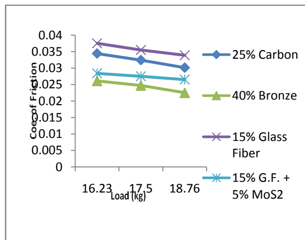
Fig. 3 C.O.F. Vs. Load for PTFE composites under wet condition.
