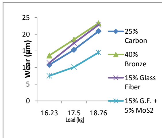
Fig.2 Wear Vs. Load for PTFE composites under wet condition.
